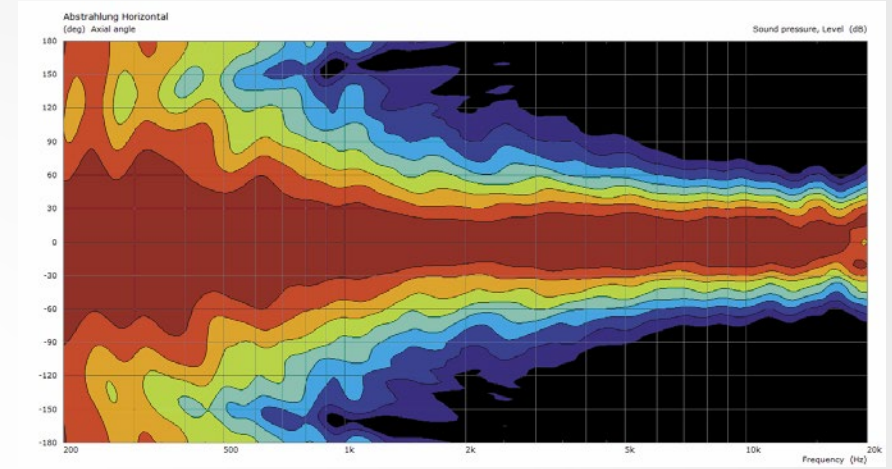
Horizontal directivity
