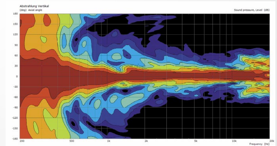
Vertical directivity
